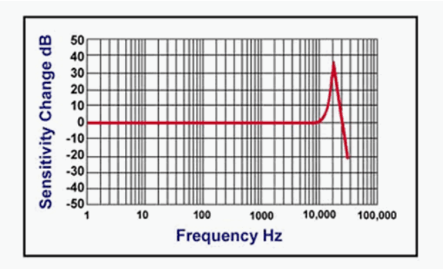
Figure 32 - 1443-ACC-IS-S Accelerometer
