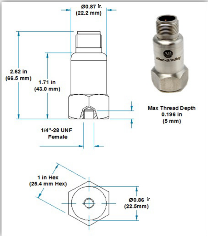
Figure 18 - 1443-ACC-LF-T Accelerometer
