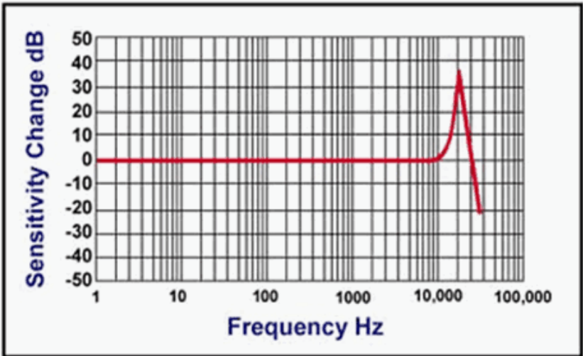
Figure 18 - 1443-ACC-LF-T Accelerometer
