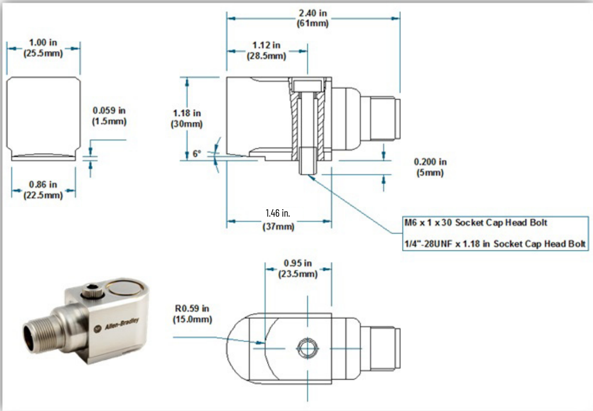
Figure 24 - 1443-ACC-V0-S Accelerometer
