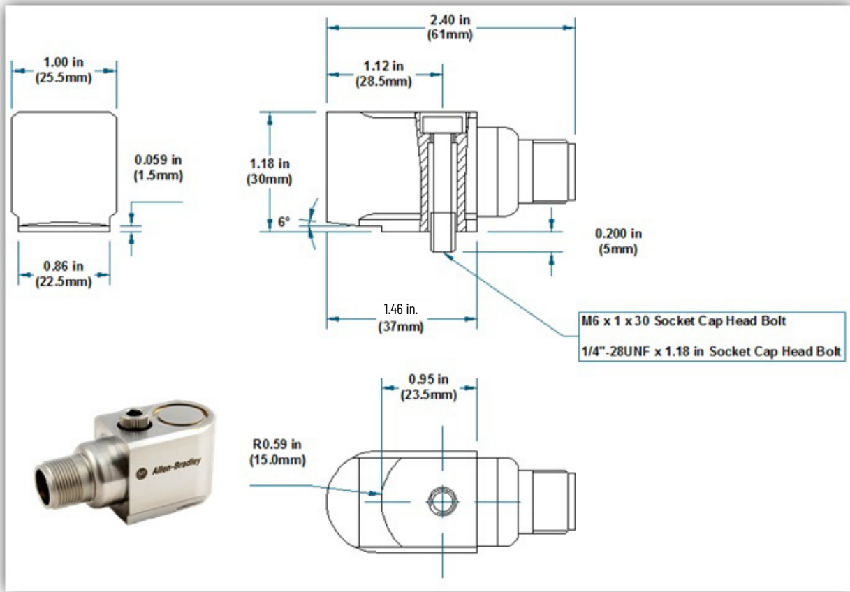
Figure 28 - 1443-ACC-AT-S Accelerometer
