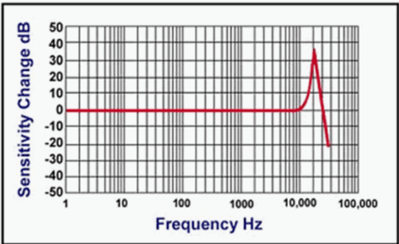
Figure 10 - 1443-ACC-GP-T16-SI Accelerometer
