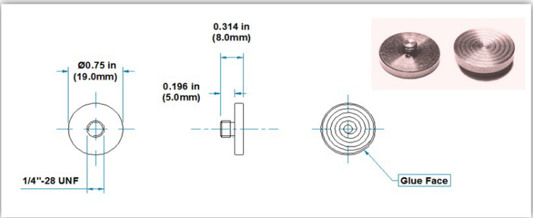
Figure 48 - 1443-PAD
