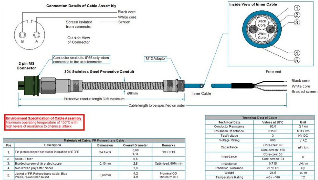
Figure 35 - 1443 -MS2IBC-50A
