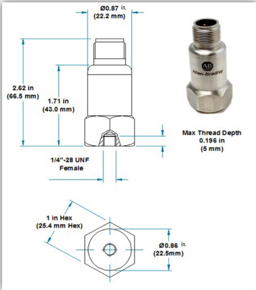
Figure 22 - 1443-ACC-V0-T Accelerometer
