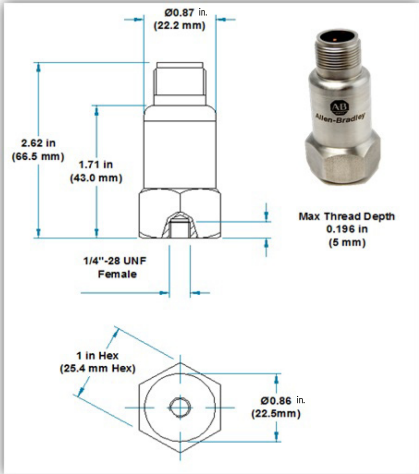
Figure 26 - 1443-ACC-AT-T Accelerometer
