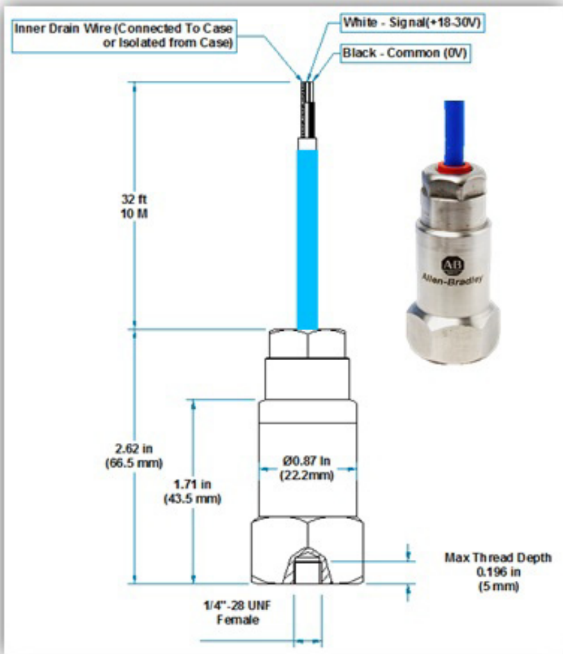
Figure 14 - 1443-ACC-GP-T16-SC Accelerometer
