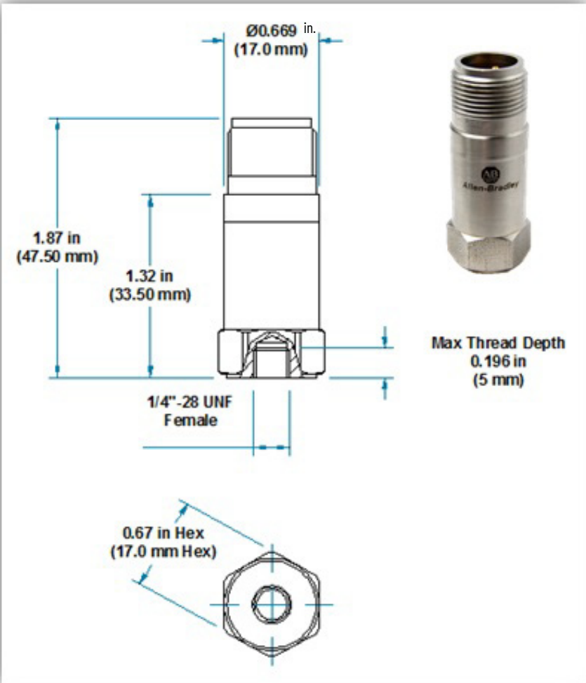
Figure 6 - 1443-ACC-GP-T Measurements
