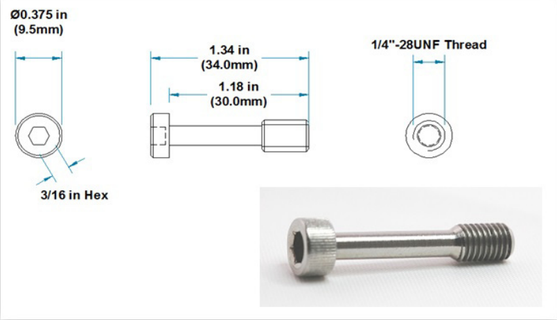
Figure 45 - 1443-BLT-125-0
