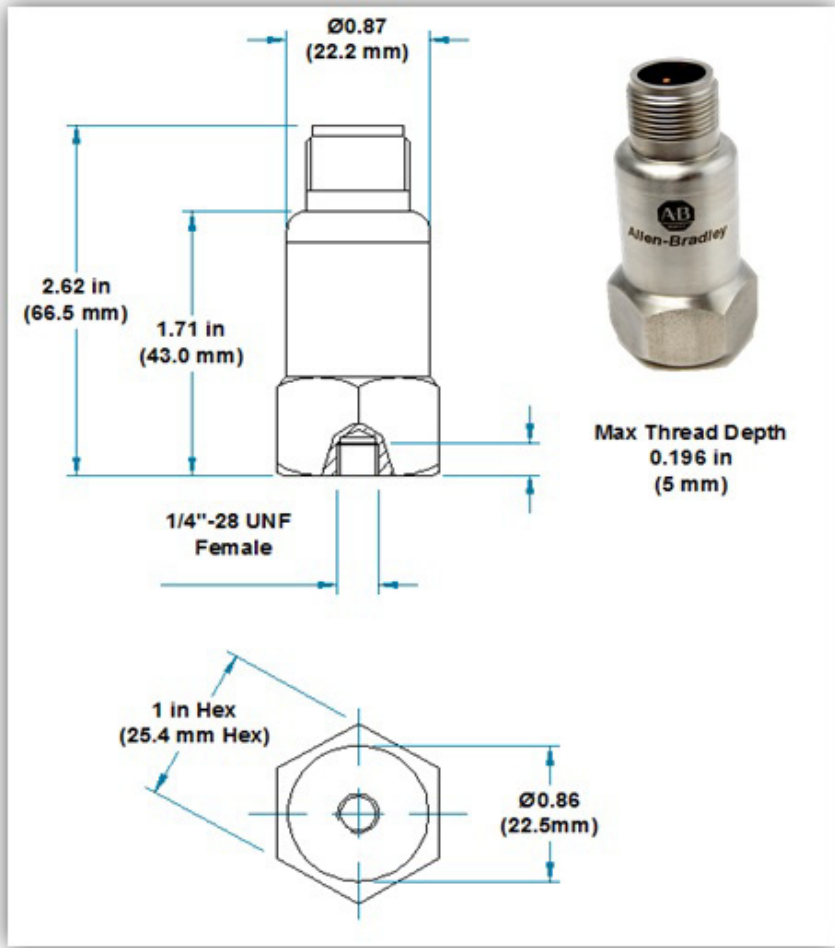
Figure 20 - 1443-ACC-HF-T Accelerometer
