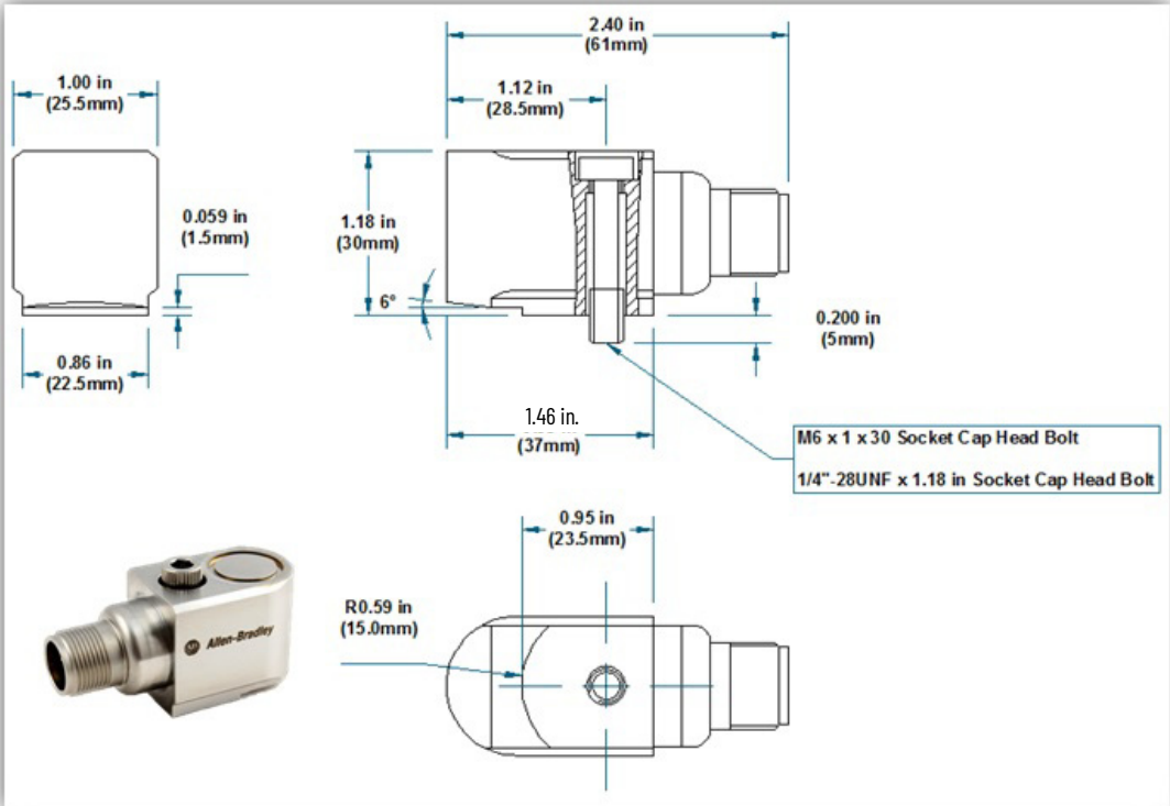
Figure 32 - 1443-ACC-IS-S Accelerometer
