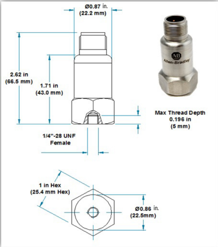
Figure 30 - 1443-ACC-IS-T Accelerometer
