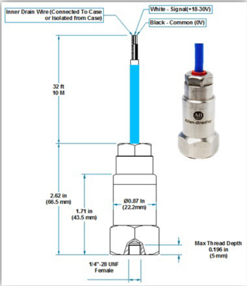
Figure 16 - 1443-ACC-GP-T32-SC Accelerometer
