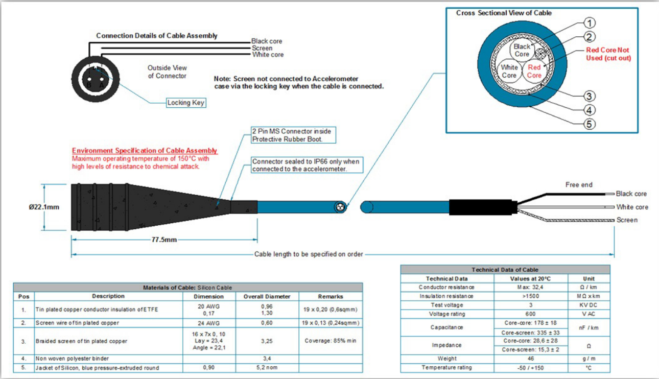
Figure 34 - 1443-CBL-MS2GBC
