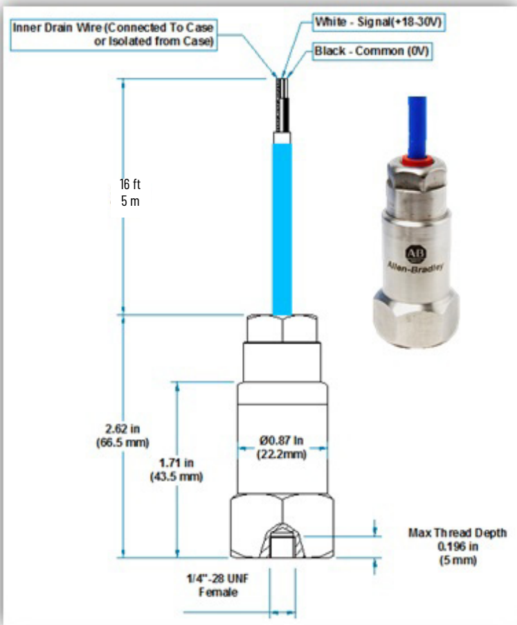
Figure 10 - 1443-ACC-GP-T16-SI Accelerometer
