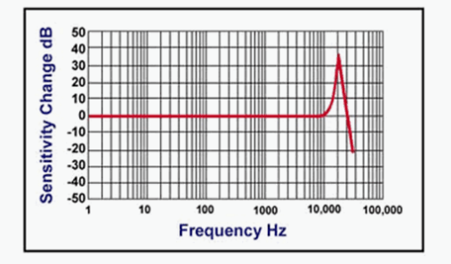
Figure 30 - 1443-ACC-IS-T Accelerometer
