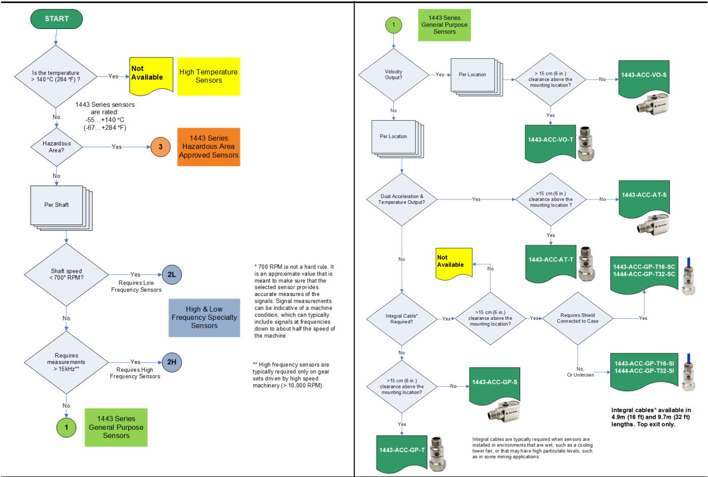
Figure 4 - Sensor Selection Flowchart
