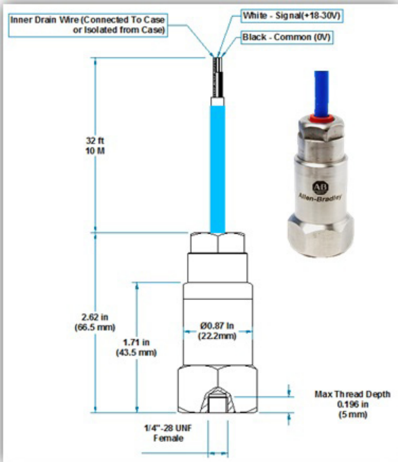
Figure 12 - 1443-ACC-GP-T32-SI Accelerometer
