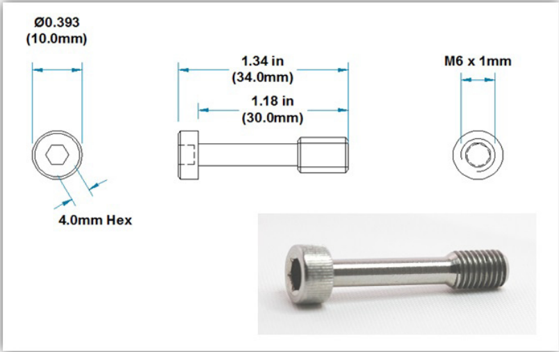
Figure 46 - 1443-BLT-125-M6
