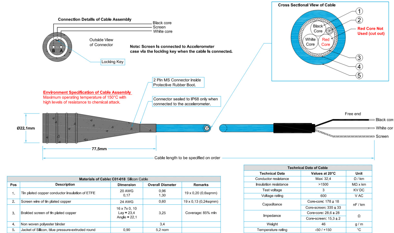
Figure 35 - 1443 -MS2IBC-50A
