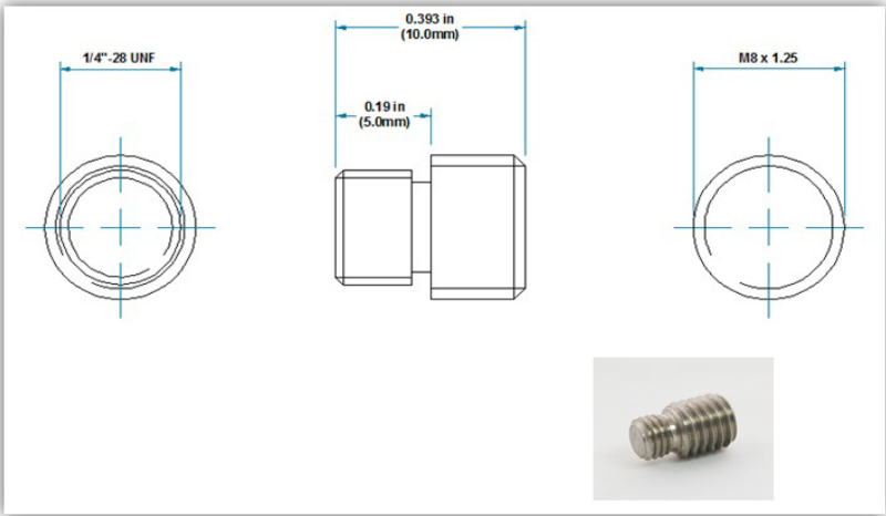
Figure 44 - 1443-STD-0-M8
