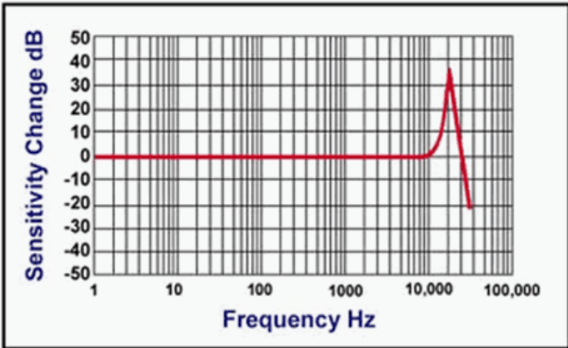
Figure 12 - 1443-ACC-GP-T32-SI Accelerometer
