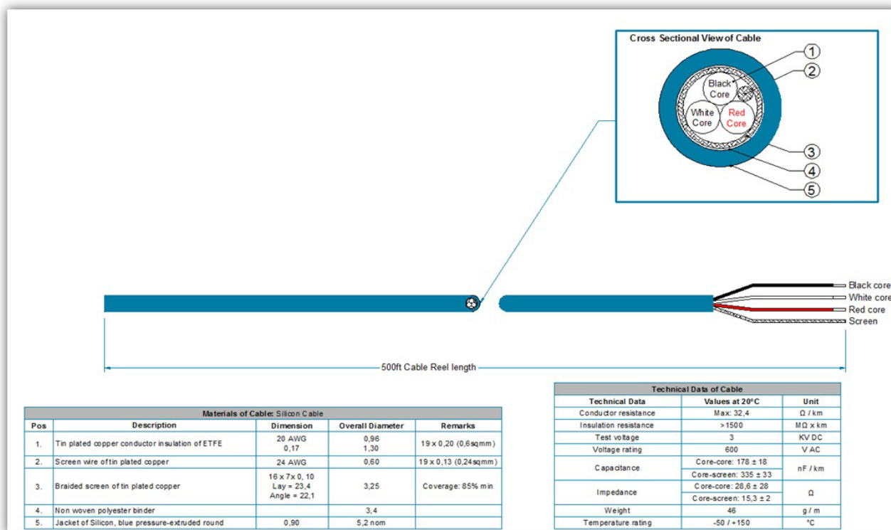
Figure 36 - 1443-CBL-BC3BC-500
