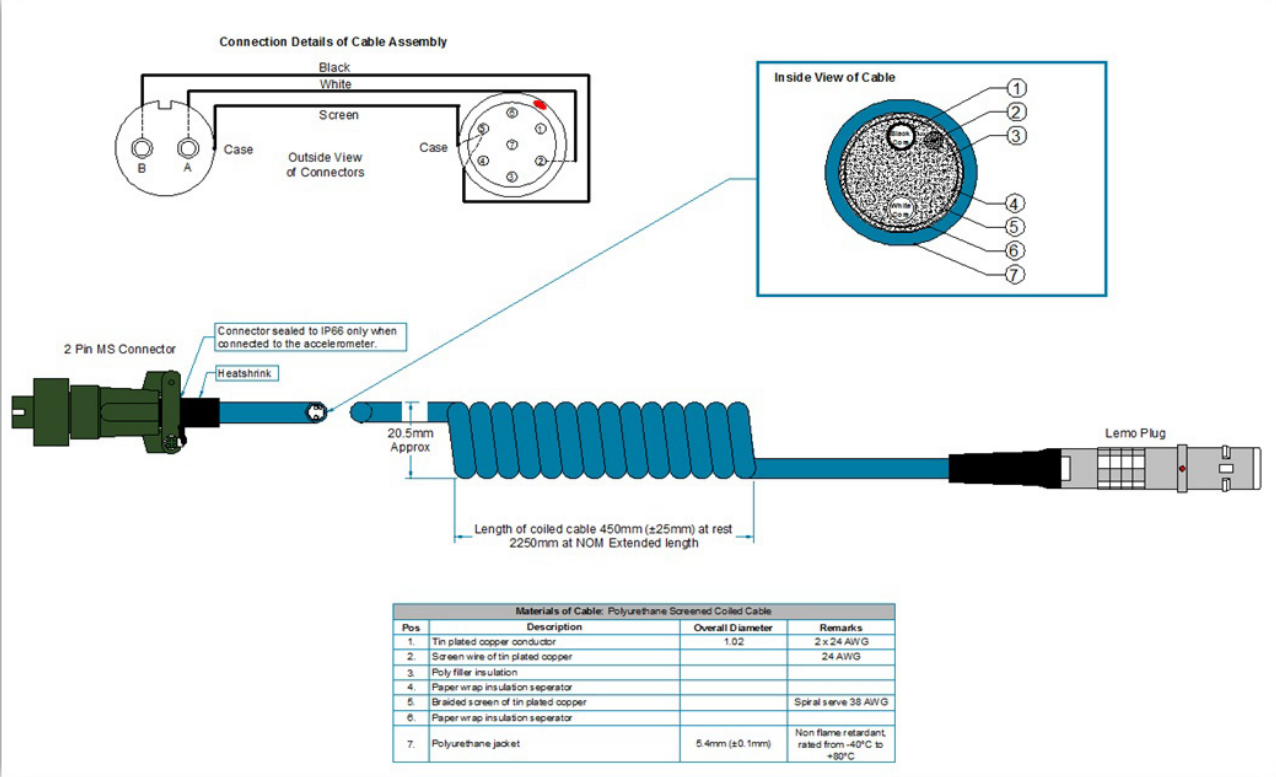
Figure 38 - 1443-CBL-MSILM-6
